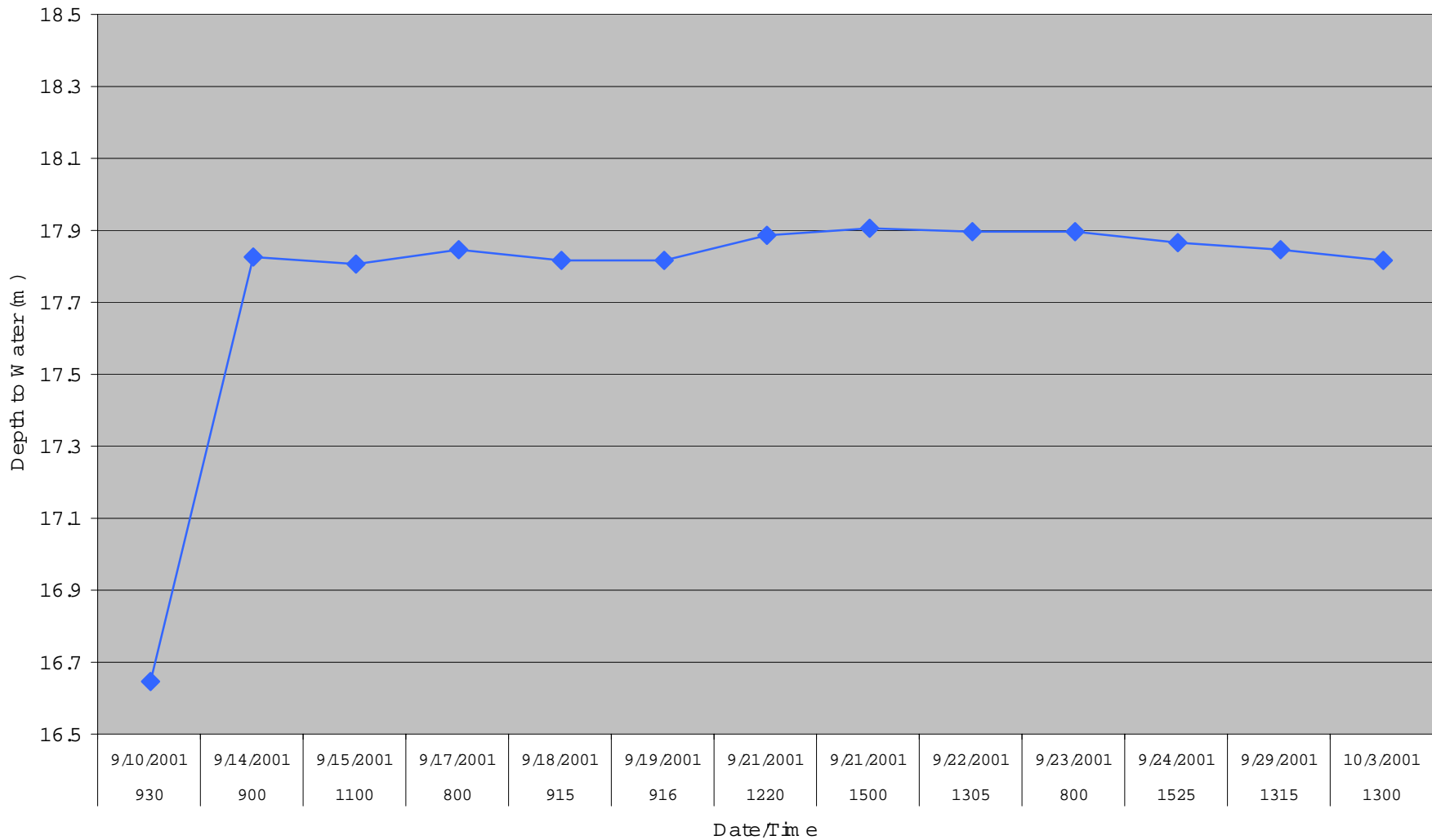
Figure C-11. Groundwater Level Hydrograph Well BCUT-1 Depth to Water vs. Time
