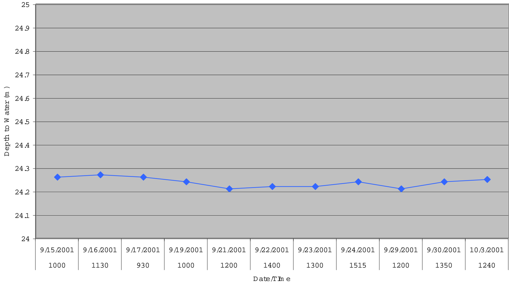
Figure C-13. Groundwater Level Hydrograph WELL BCUT-2 Depth to Water vs. Time
