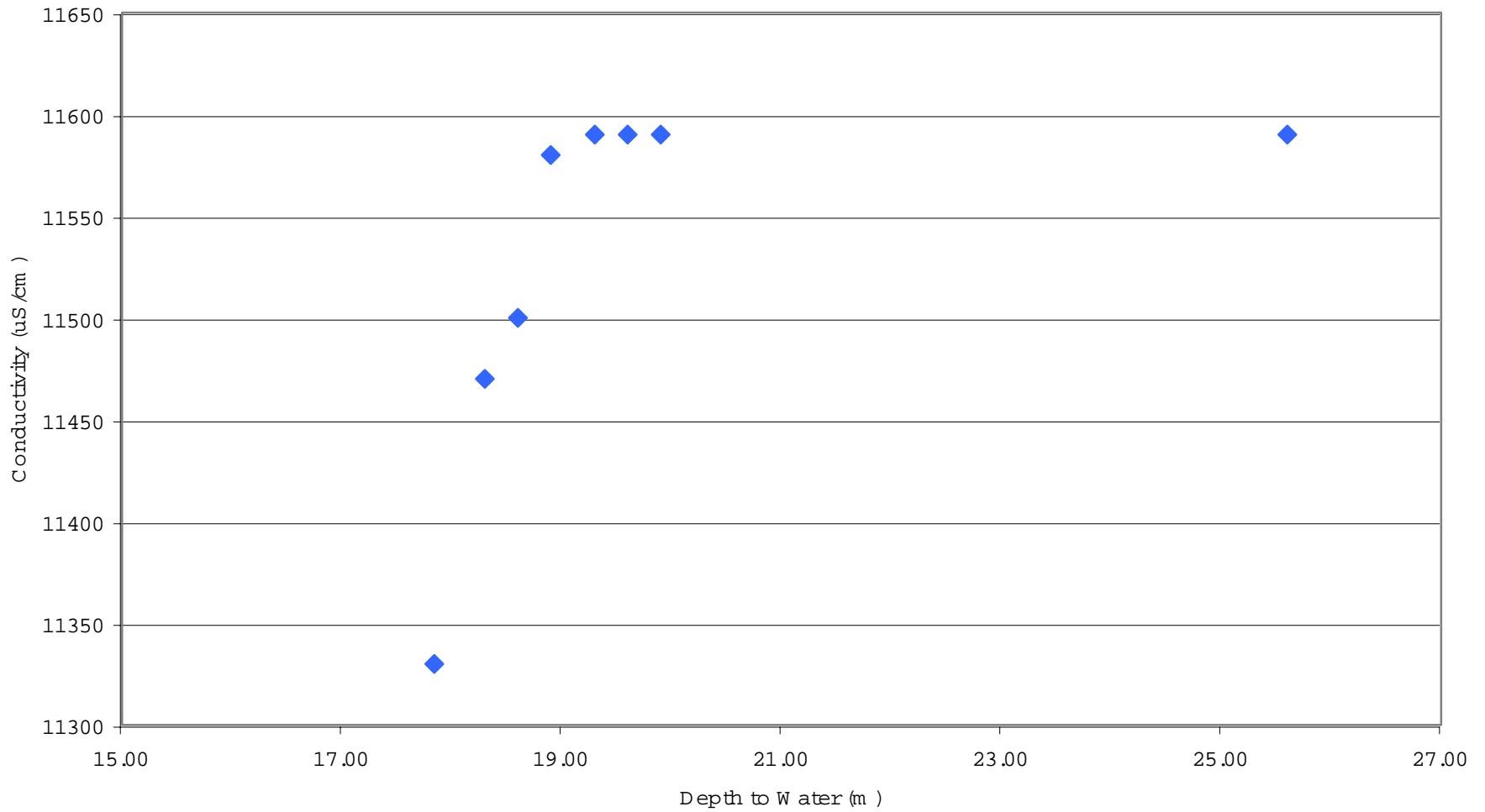
Figure C-6. Vertical Conductivity Profile Well BCUT-1 Depth to Water vs. Conductivity
