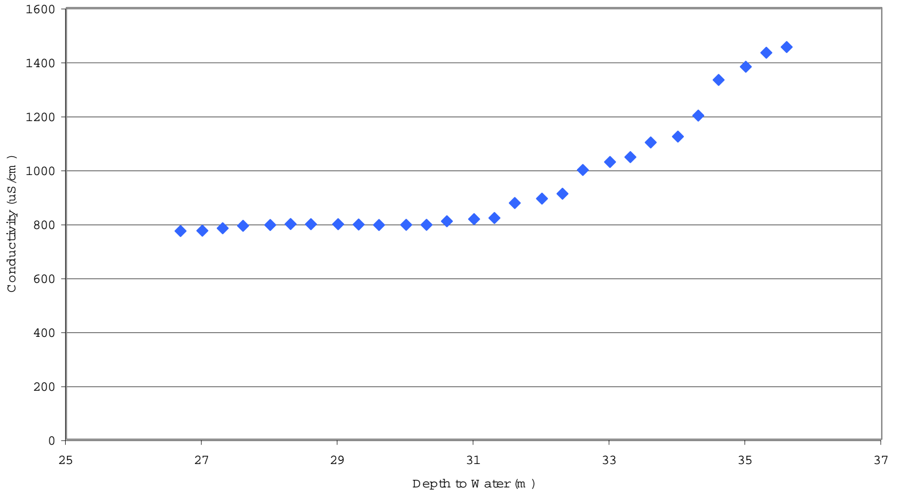
Figure C-10. Vertical Conductivity Profile Well BCUT-4 Depth to Water vs. Conductivity
