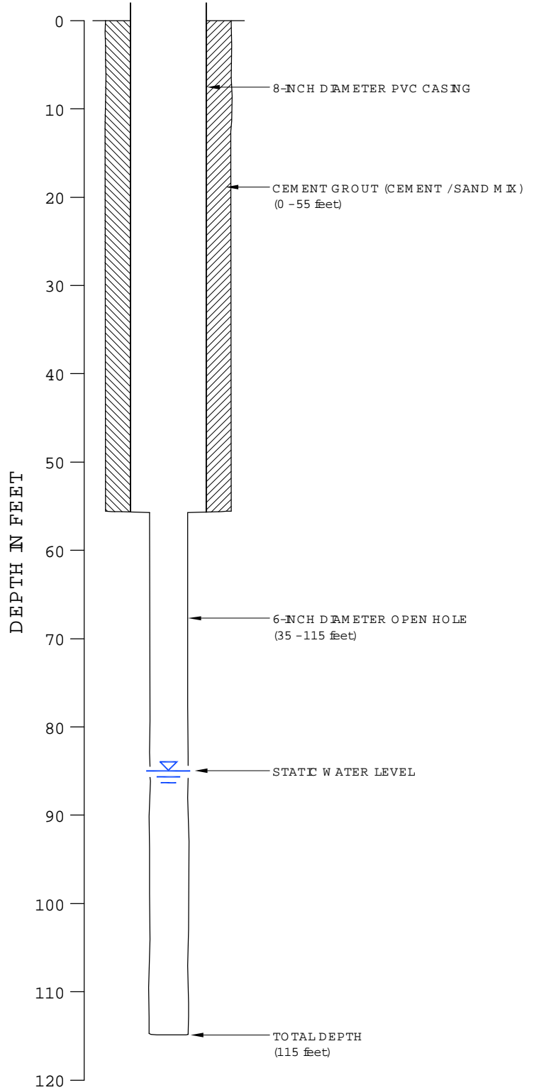
Figure C-5 TEST WELL BCUT-4 ISLA DE UTILA, HONDURAS
