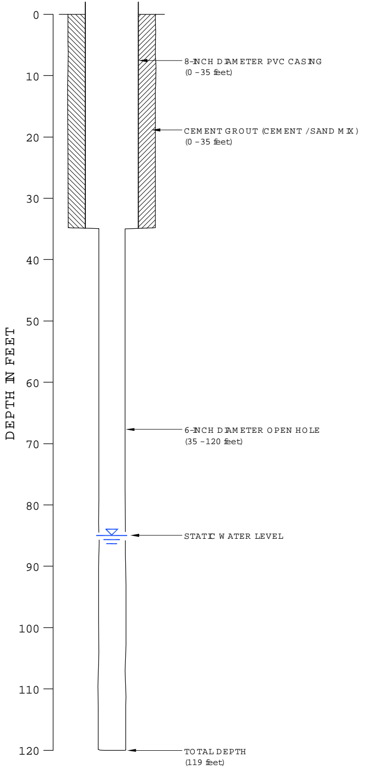
Figure C-4 TEST WELL BCUT-3 ISLA DE UTILA, HONDURAS
