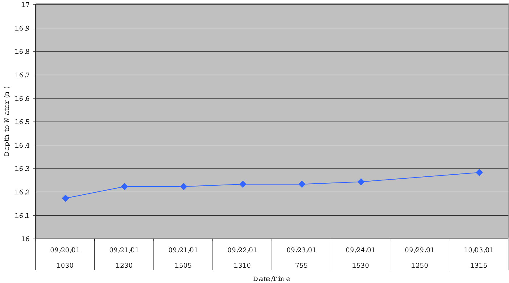
Figure C-12. Groundwater Level Hydrograph WELL BCUT-1A Depth to Water vs. Time
