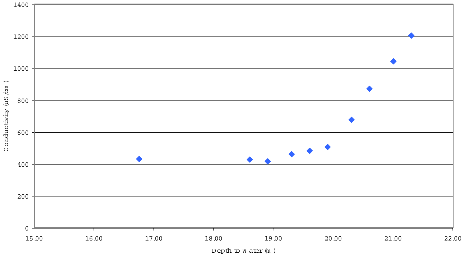
Figure C -7. Vertical Conductivity Profile Well BCUT -1A Depth to Water vs. Conductivity
