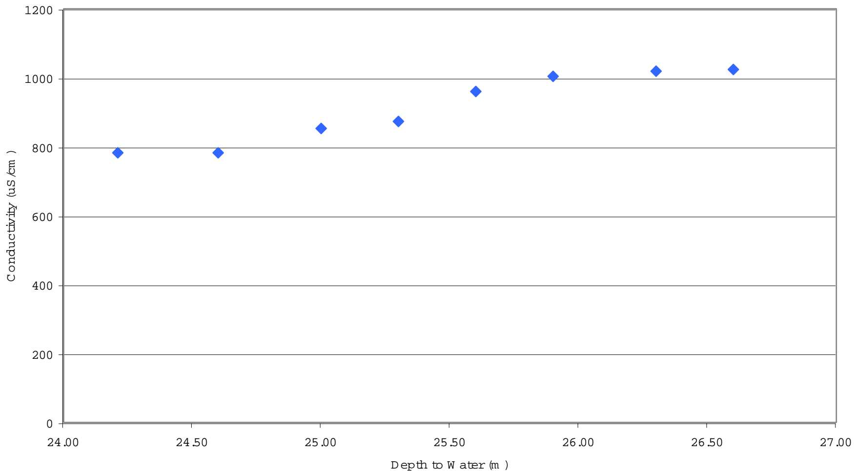
Figure C-8. Vertical Conductivity Profile Well BCUT-2 Depth to Water vs. Conductivity
