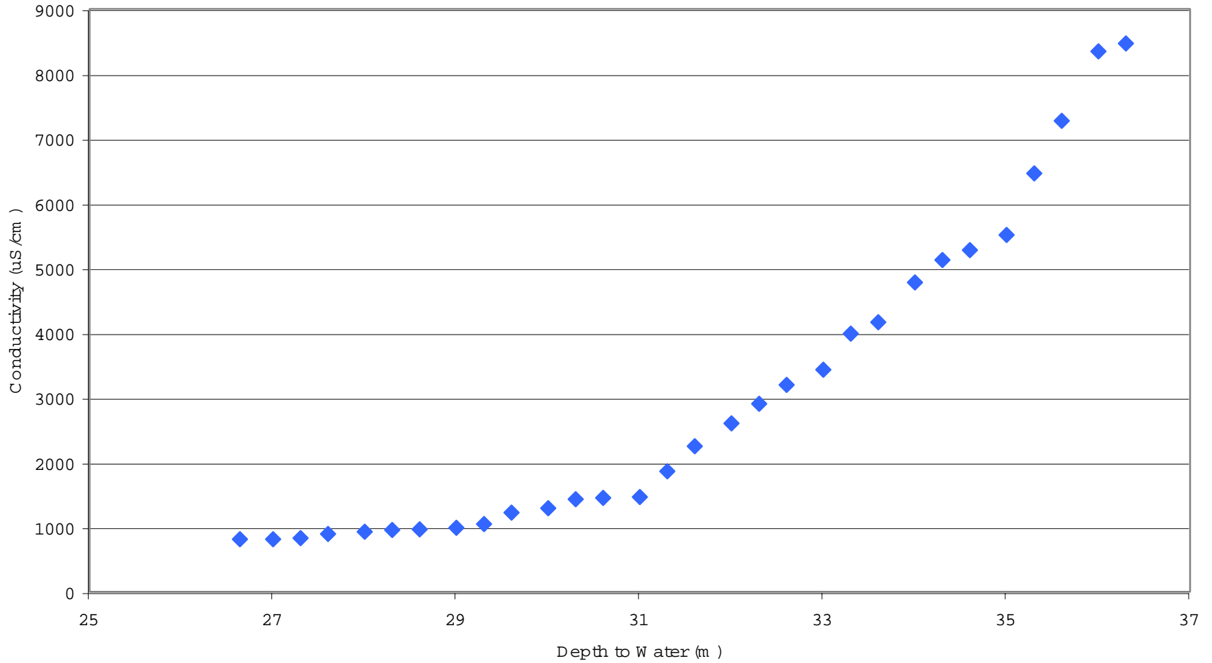
Figure C-9. Vertical Conductivity Profile Well BCUT-3 Depth to Water vs. Conductivity
