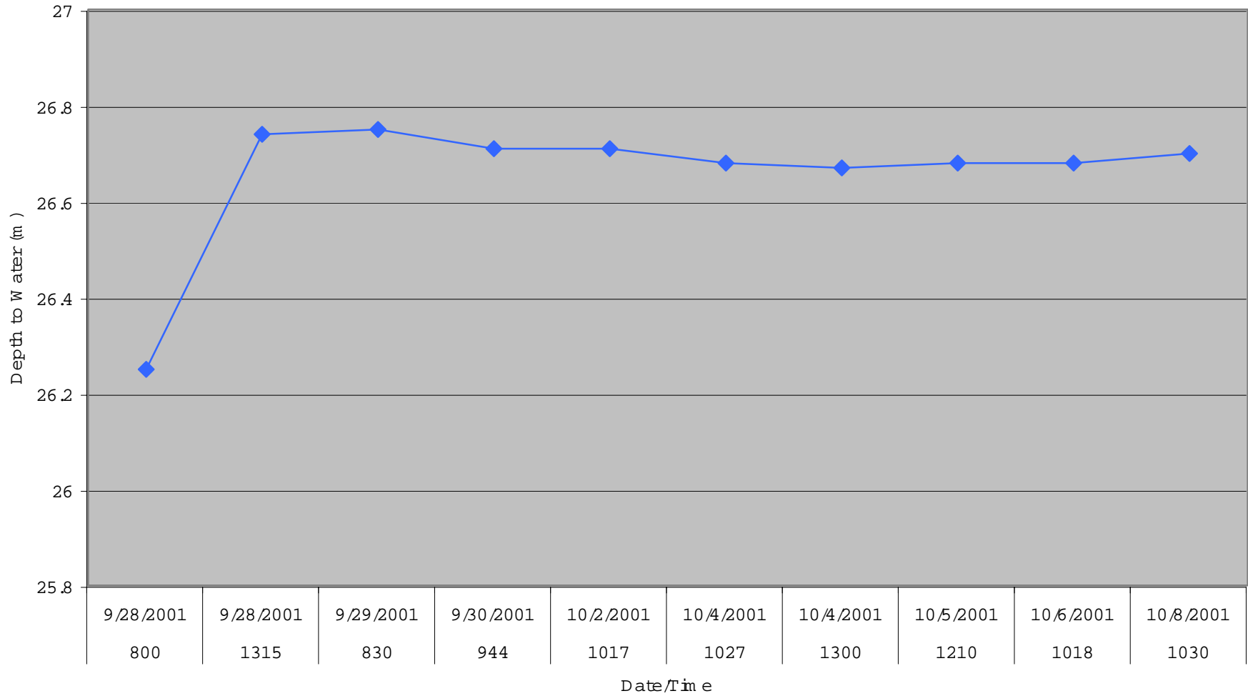
Figure C-15. Groundwater Level Hydrograph Well BCUT-4 Depth to Water vs. Time
